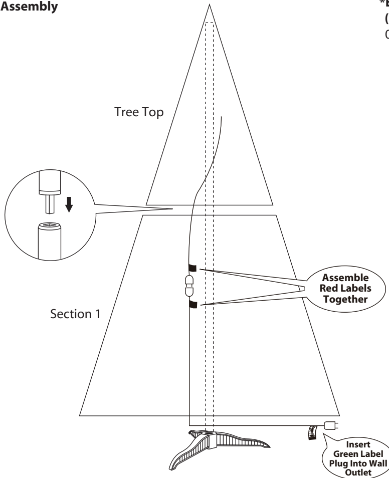
Fig. B - Tree and Light Assembly
