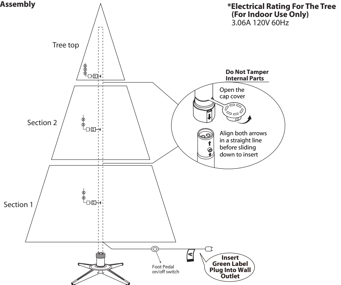
Fig. B - Tree and Light Assembly
