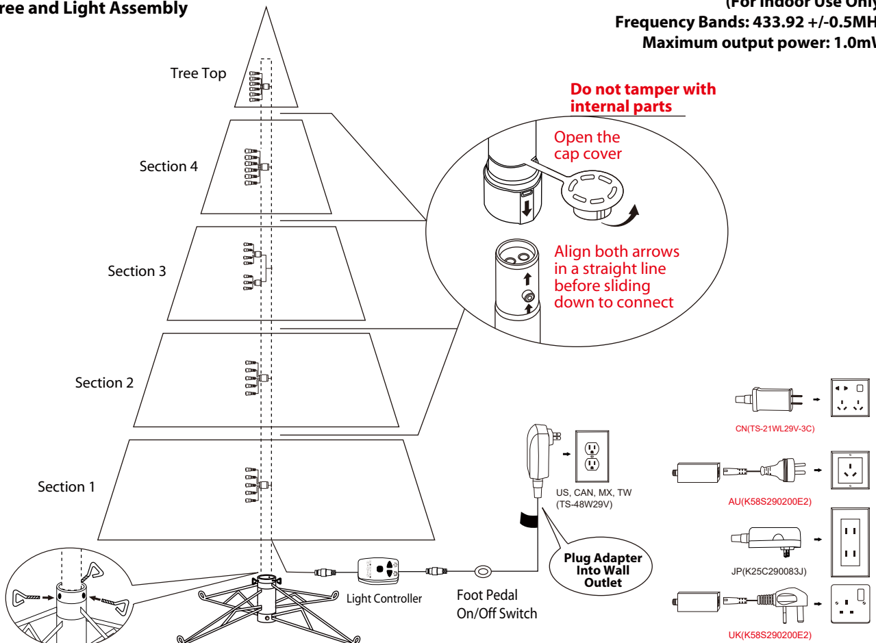
Fig. B - Tree and Light Assembly
