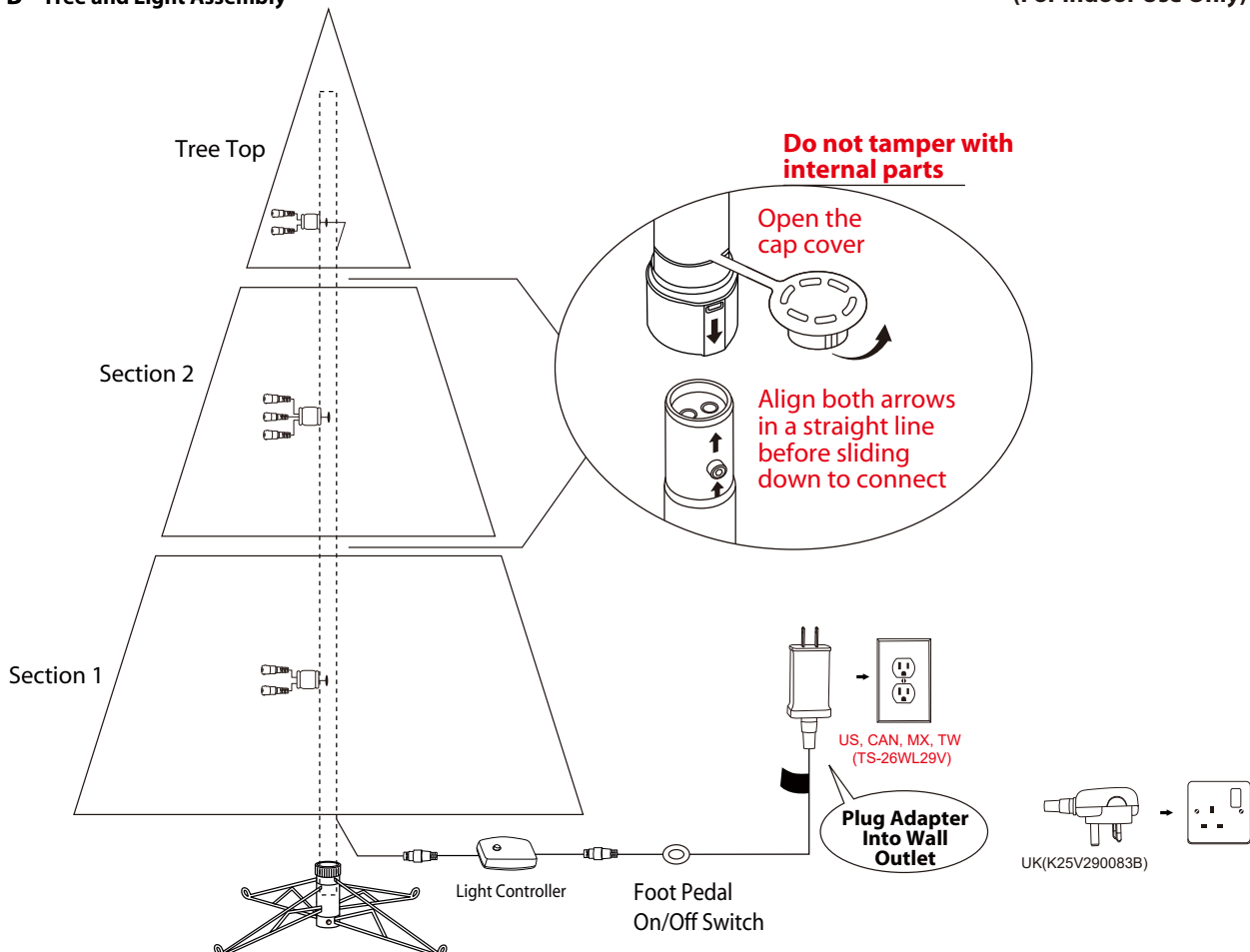
Fig. B - Tree and Light Assembly
