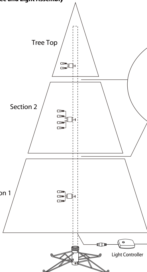
Fig. B - Tree and Light Assembly
