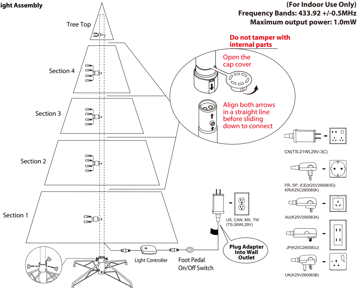
Fig. B - Tree and Light Assembly
