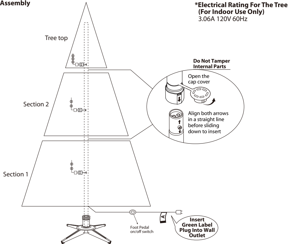
Fig. B - Tree and Light Assembly
