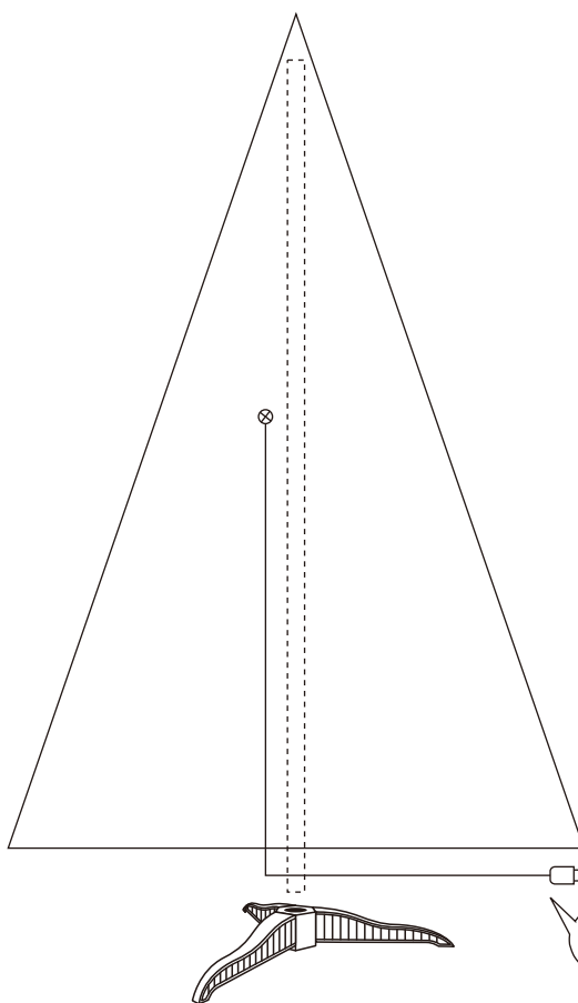
Fig. B - Tree and Light Assembly
