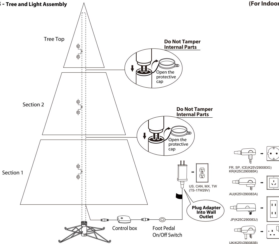
Fig. B - Tree and Light Assembly
