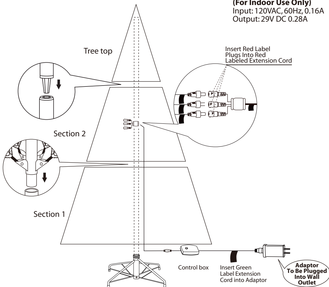
Fig. B - Tree and Light Assembly
