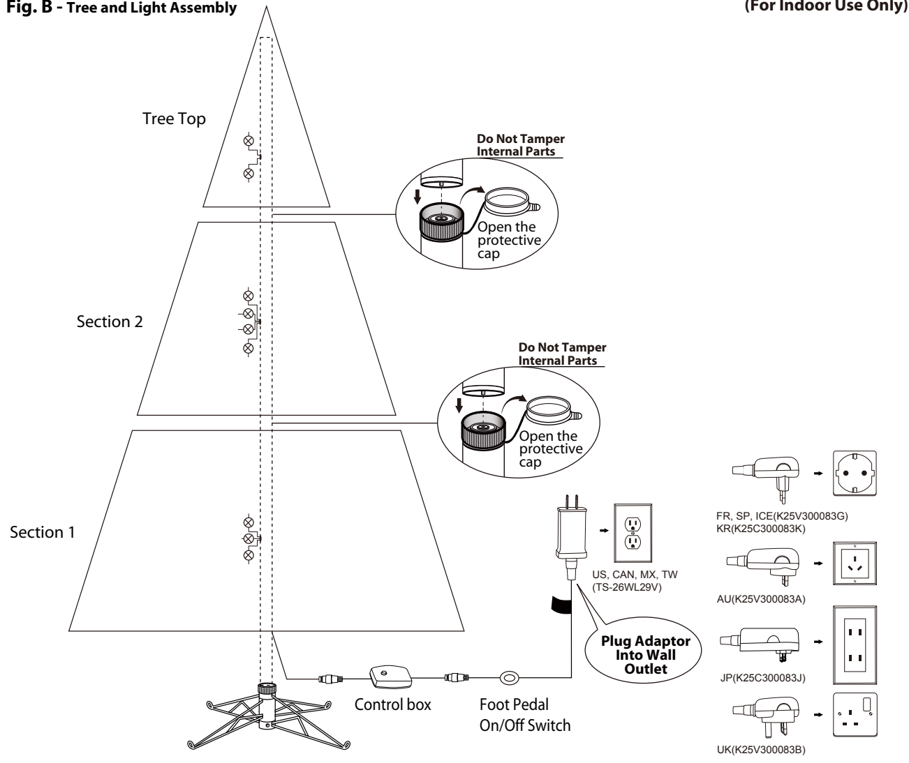
Fig. B - Tree and Light Assembly
