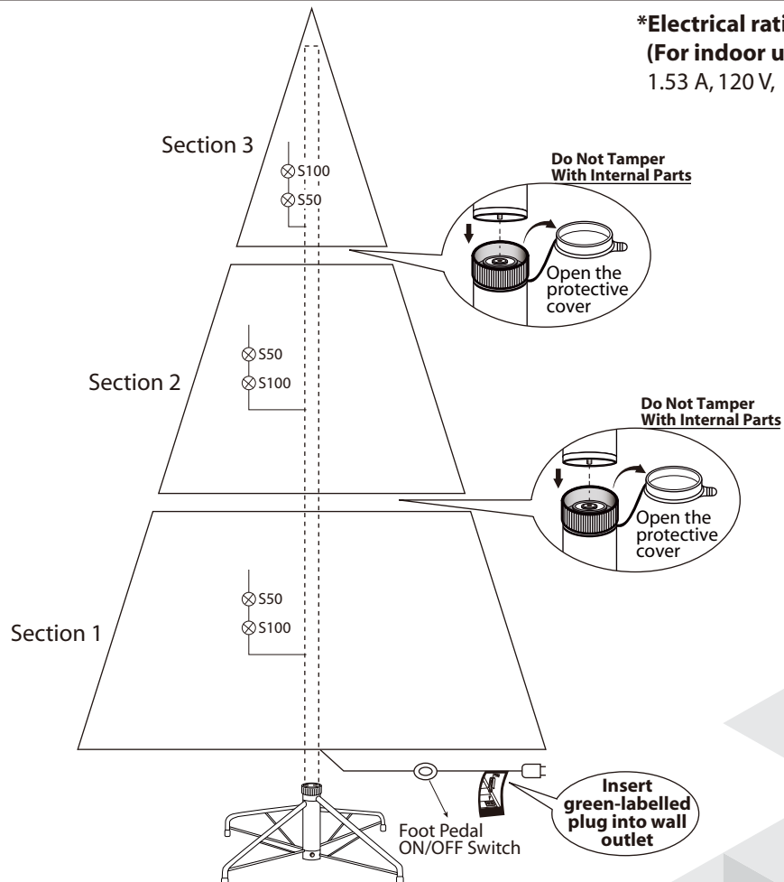
Fig. B - Tree and Light Assembly
