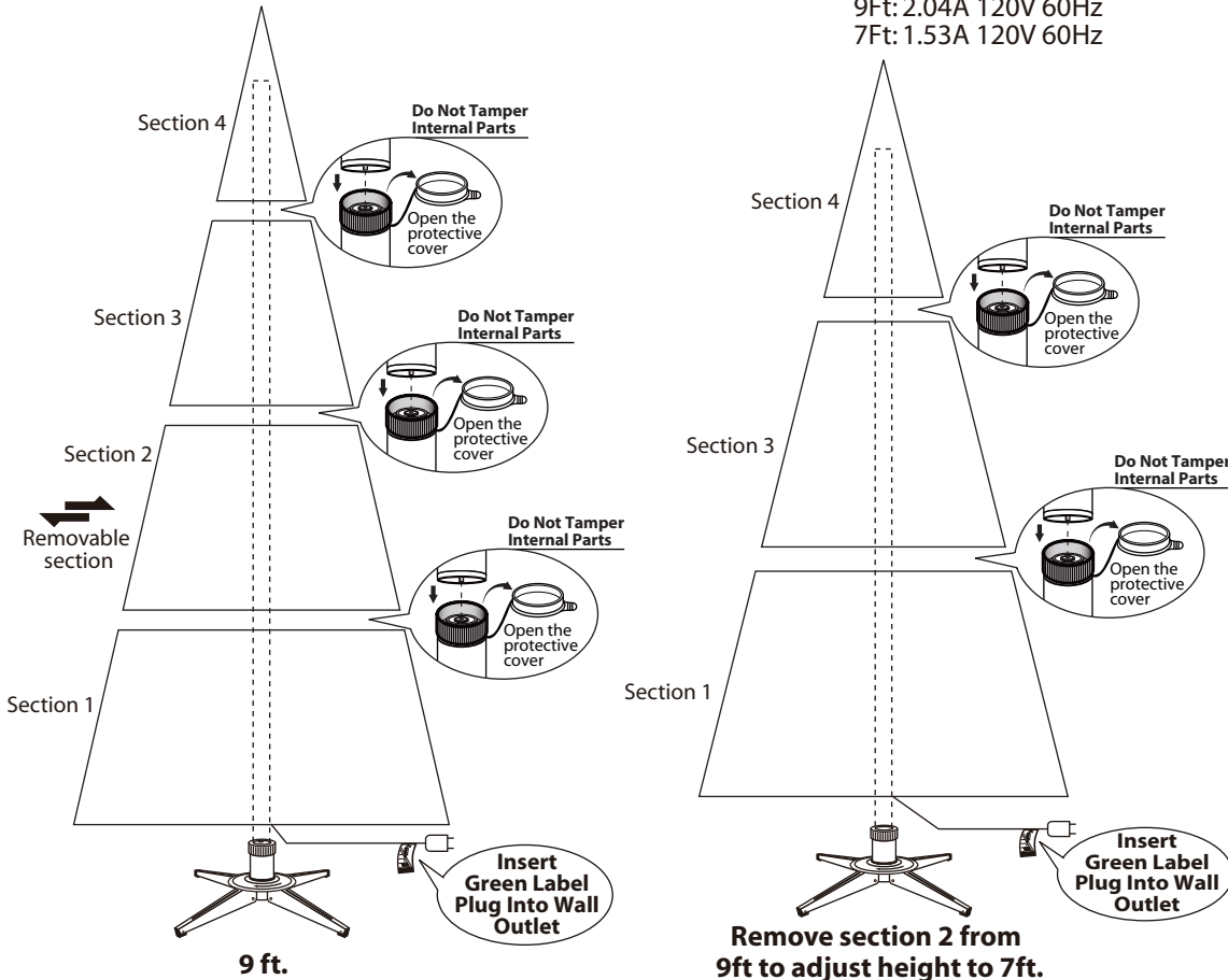
Fig. B - Tree and Light Assembly
