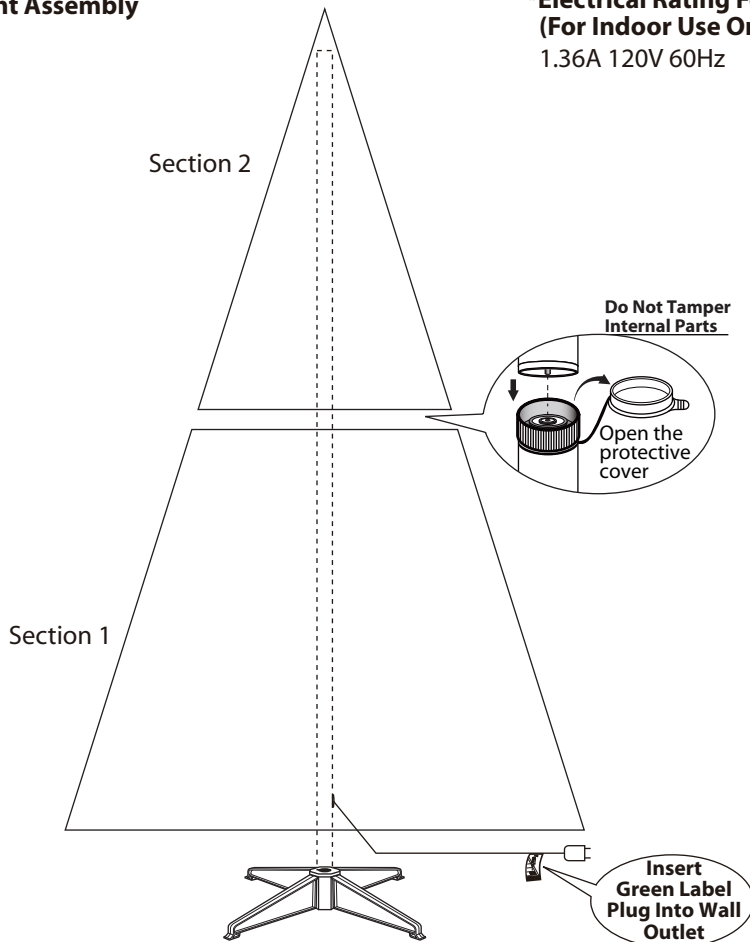
Fig. B - Tree and Light Assembly
